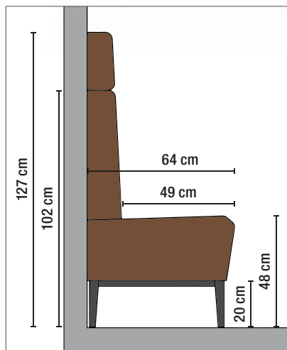
Dimensions of the bench system
