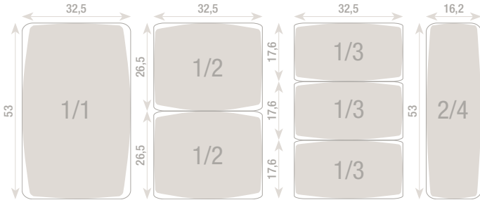
Plat buffet - "Buffet" serving dish
