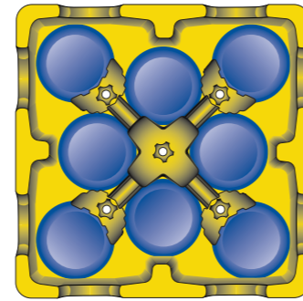
ADS4 Layout for 19.05 cm round plates and 15.24 cm square plates
