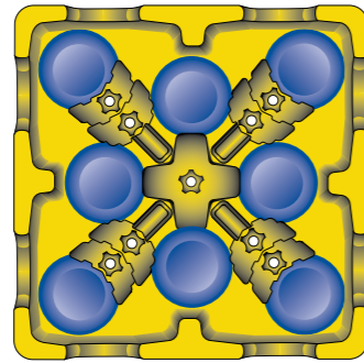
ADS8 Layout for 16.51 cm round plates
